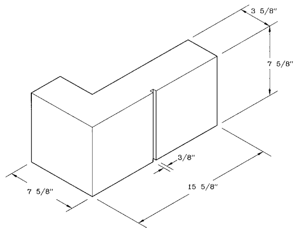
4x8x16 Scored Return
