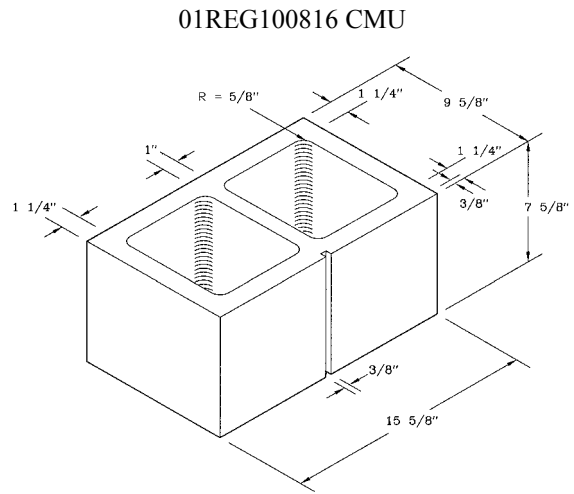
10x8x16 Scored CMU
