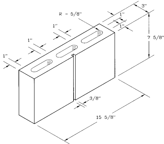
3x8x16 Scored CMU (Actual Width)
