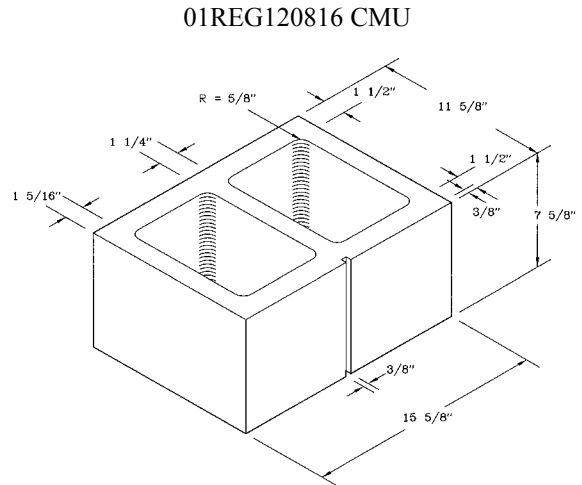
12x8x16 Scored CMU
