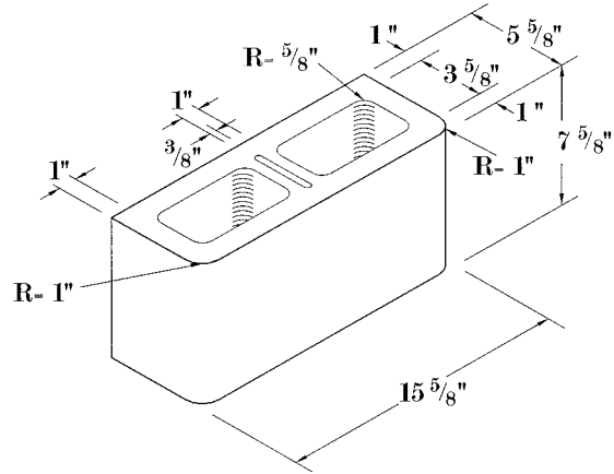
6x8x16 Bullnose Pier
