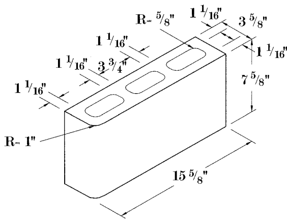
4x8x16 Bullnose CMU
