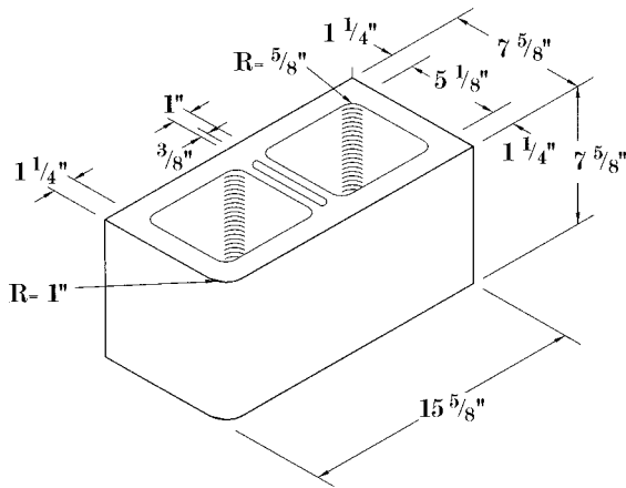
8x8x16 Bullnose CMU
