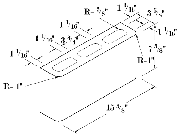
4x8x16 Bullnose Pier
