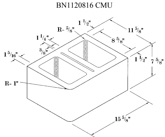
12x816 Bullnose CMU
