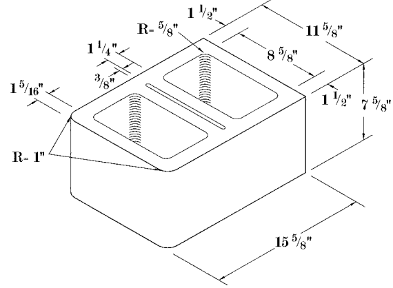
12x8x16 Double Bullnose
