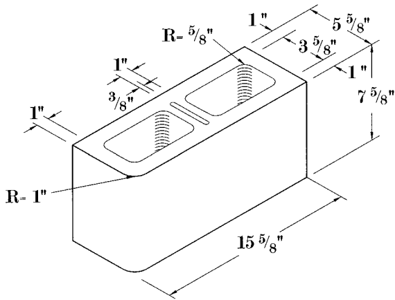
6x8x16 Bullnose CMU
