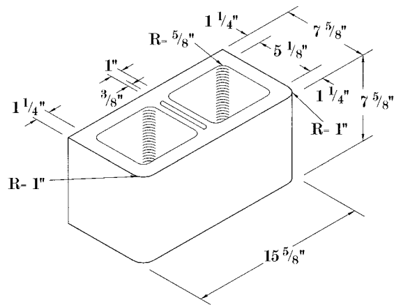
8x8x16 Bullnose Pier
