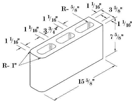
4x8x16 Double Bullnose
