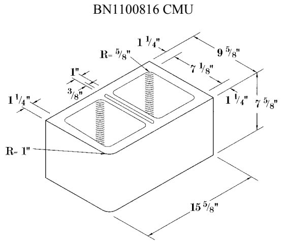
10x8x16 Bullnose CMU
