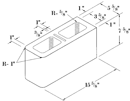
6x8x16 Double Bullnose
