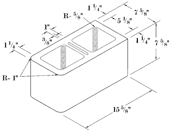
8x8x16 Double Bullnose
